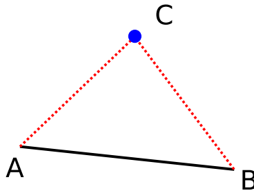
Figure 154: Example of the triangle inequality theorem
